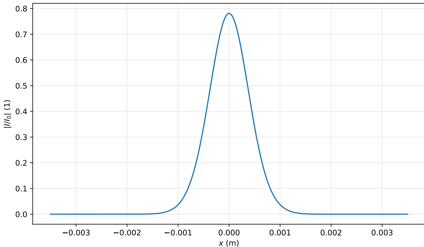
Intensity profile I(x, y = 0, z = 1.353m)/I_0 , P_{in}=0.2P_{cr} , artificial time
